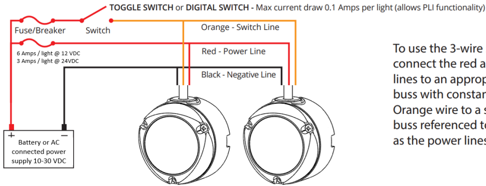
Figure 1: Kraken wiring diagram. Basic installation.
